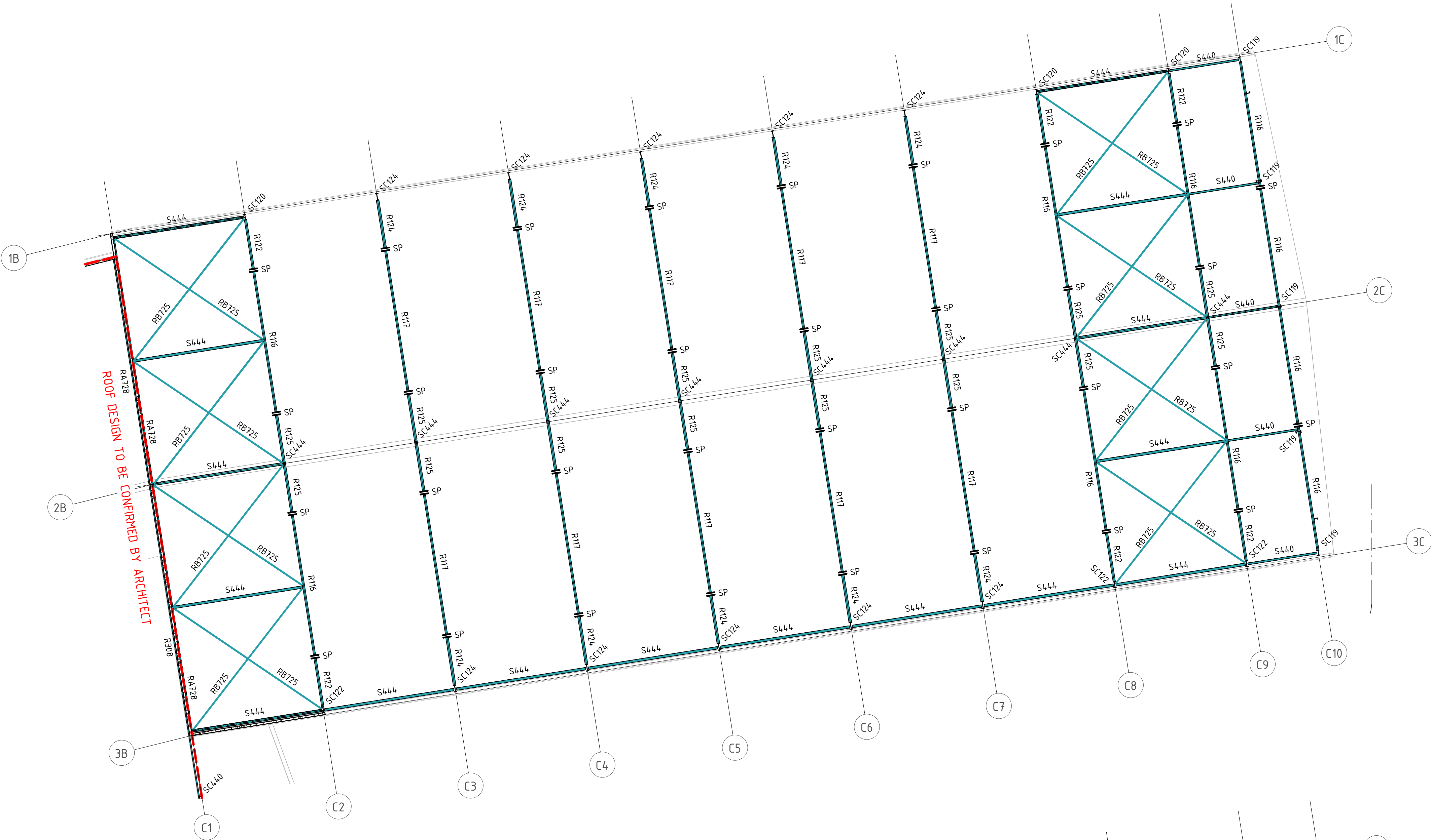
UPPER FRAMING ROOF PLAN - PART 3
